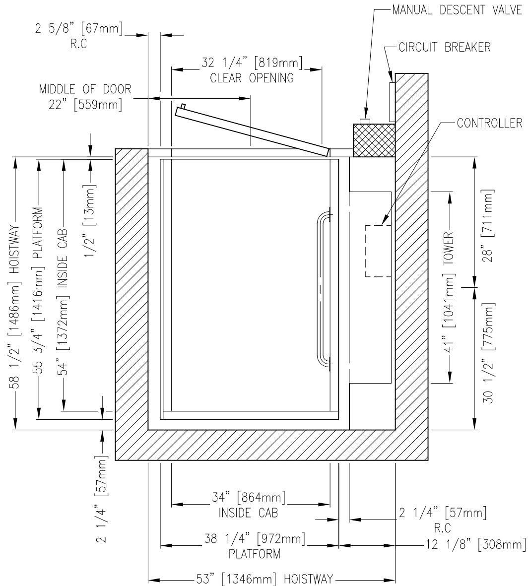
HOISTWAY LAYOUT
