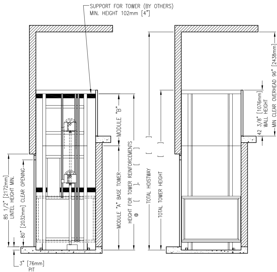
ELEVATION VIEW (MECHANICAL ELEMENTS)
